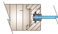
Glass stop flush
