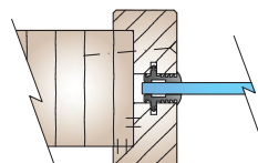
Glass stop rabbet
